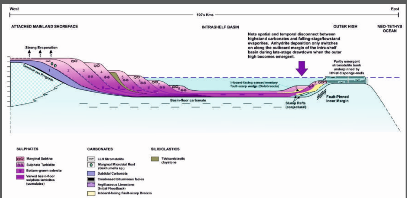
Simplified Regional-Scale Stratal Architecture (~500km-long schematic dip-section based on seismic, well and outcrop datasets)
