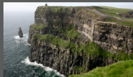
Deltaic and Turbidite Deposystems
