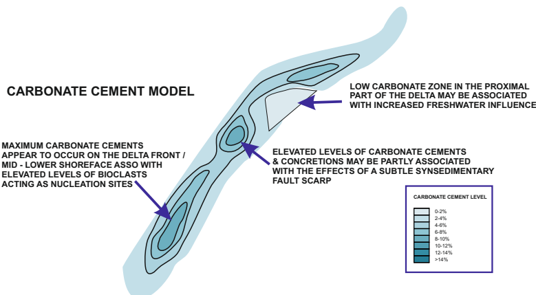
Example Modelling of Cement Distribution in a Shoreface Sandstone Reservoir (Length of sand body ~30km)
