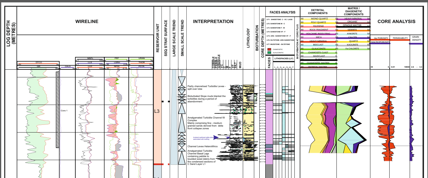
Example 1:200 Core Summary Chart Extract
